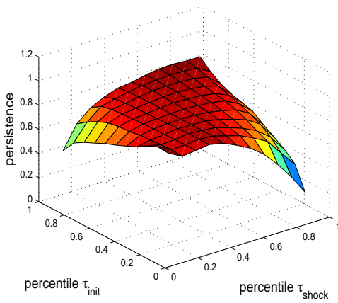
(c) Bandwidth=.3
